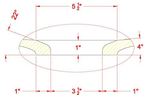
Drain Detail
